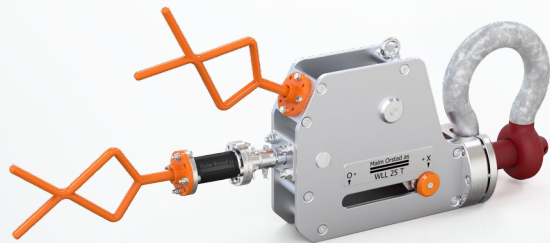
ROV Shackle with Fishtail
