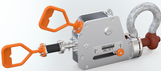
ROV Shackle with D-handle
